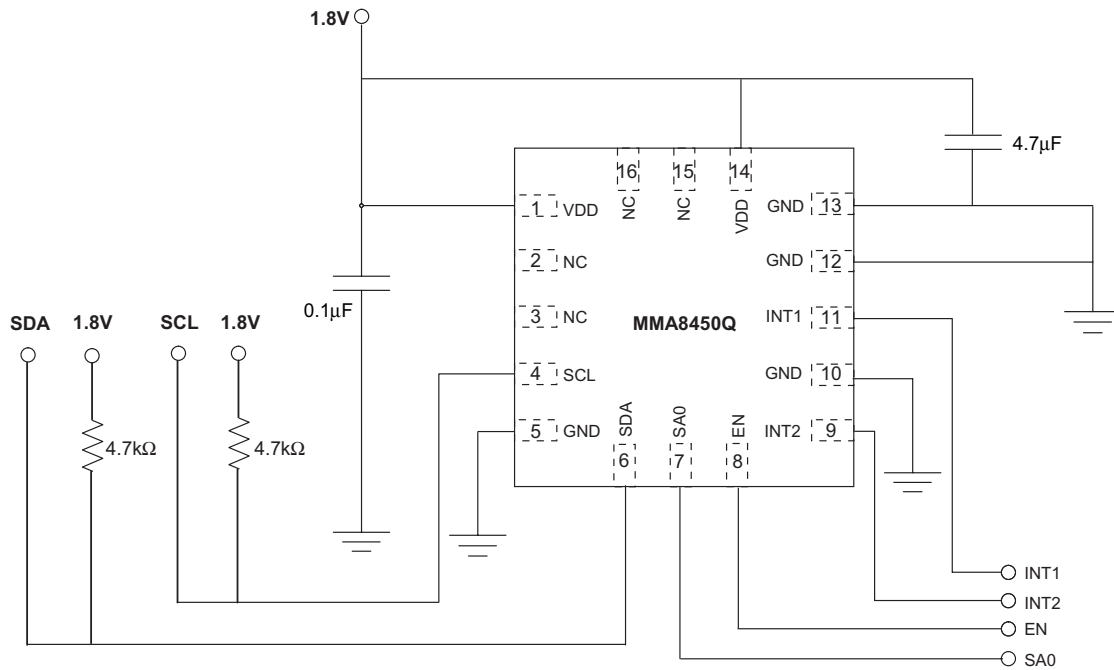
Figure 3. Application Diagram
